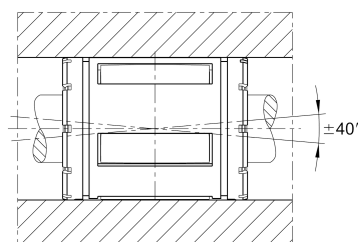
KS30, 40, 50 KSO30, 40, 50
